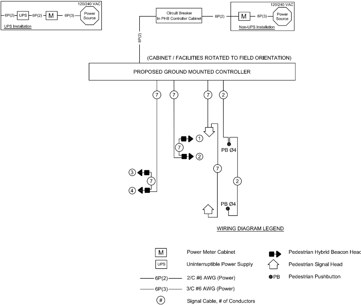
Figure 16.7 Pedestrian Hybrid Beacon Wiring Diagram Example
