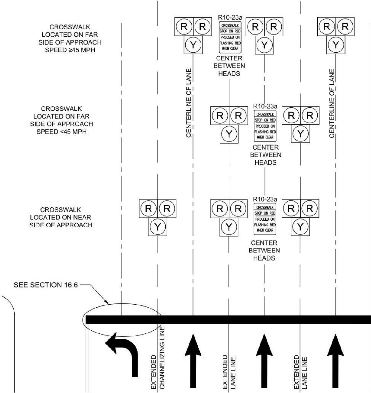
Figure 16.6 Pedestrian Hybrid Beacon Head Alignment Intersection Crossing Four Approach Lanes
