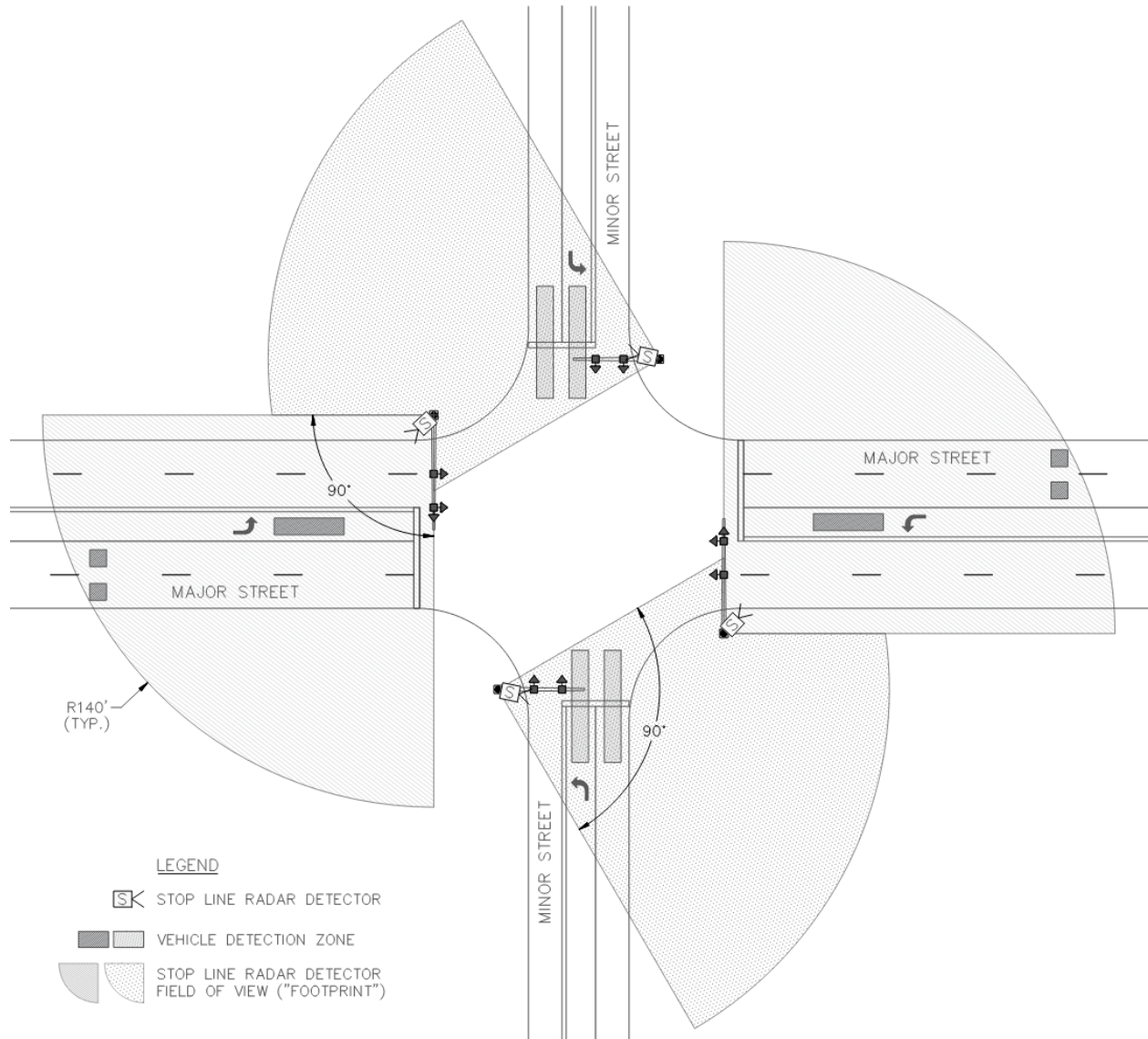
FIGURE 9.4 Stop Line Detector Placement Example Mast Arm Intersection Layout (Low Speed, 35 MPH or Less)
