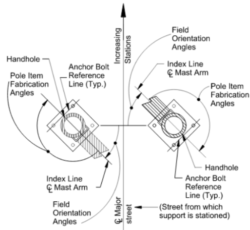
Figure 4.4 Typical Mast Arm Fabrication and Orientation Data
