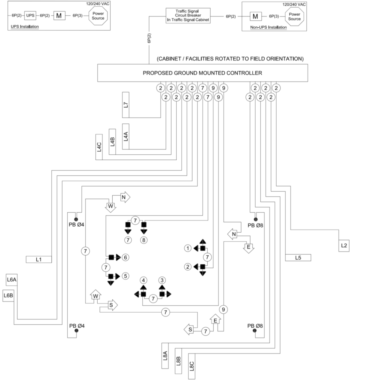
Figure 7.6 Intersection Wiring Diagram With Loop Detectors
