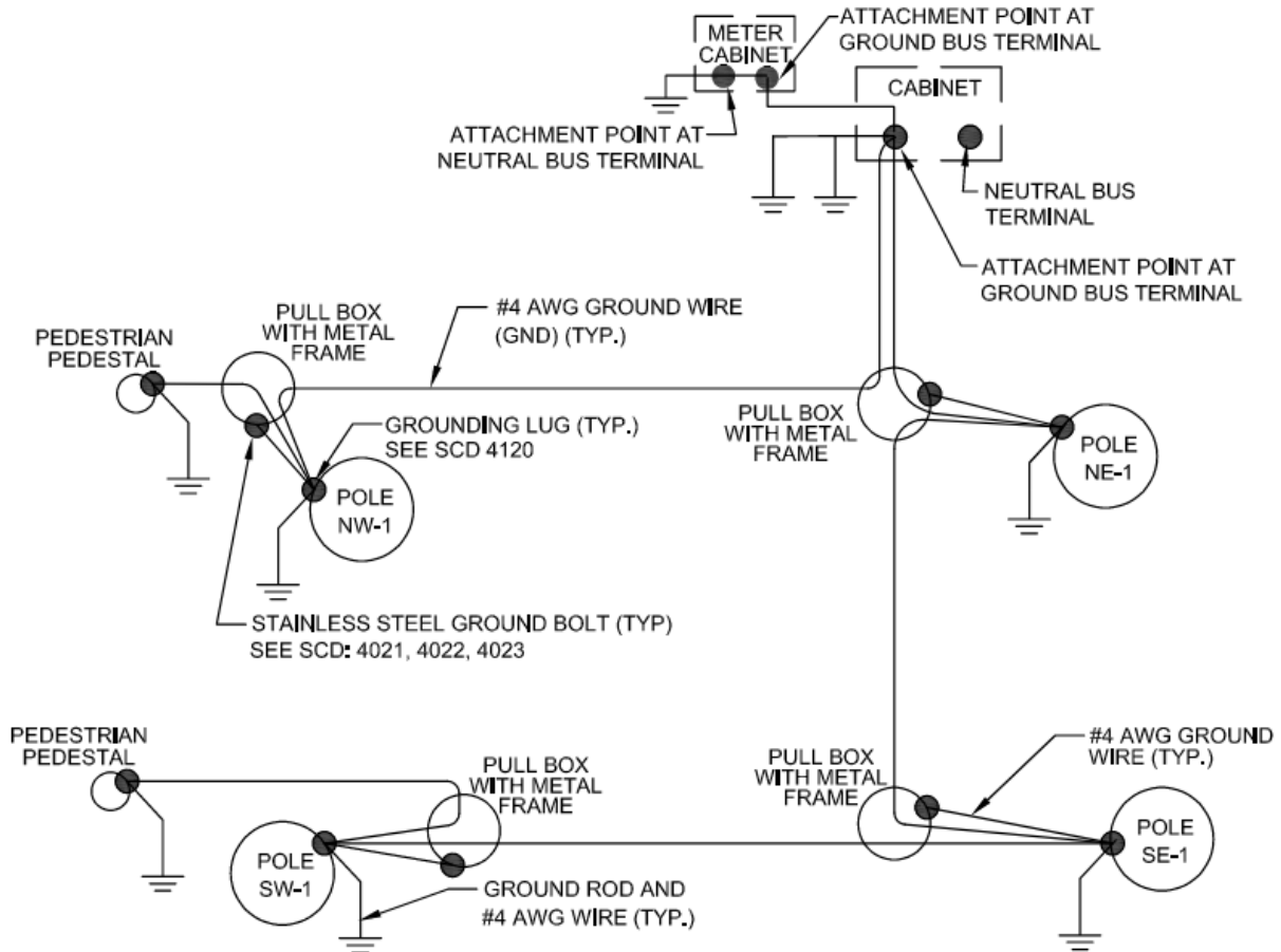
Figure 7.1 Grounding and Bonding Wiring Illustration Mast Arm Example
