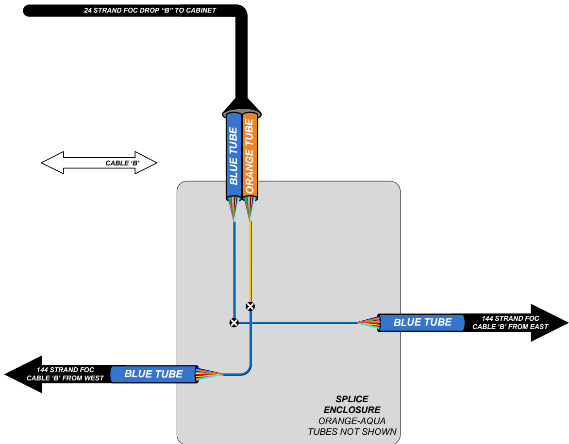
Figure 12.7 Splicing Orientation – 2 cables - East/West
