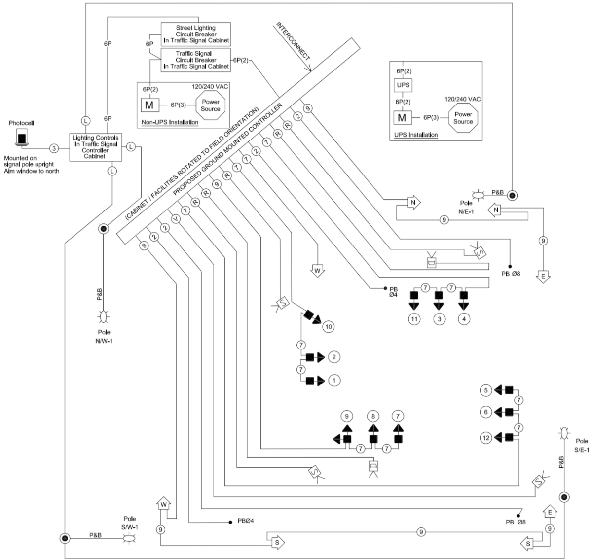
Figure 7.7 Intersection Wiring Diagram With Radar Detection and Combination Lighting
