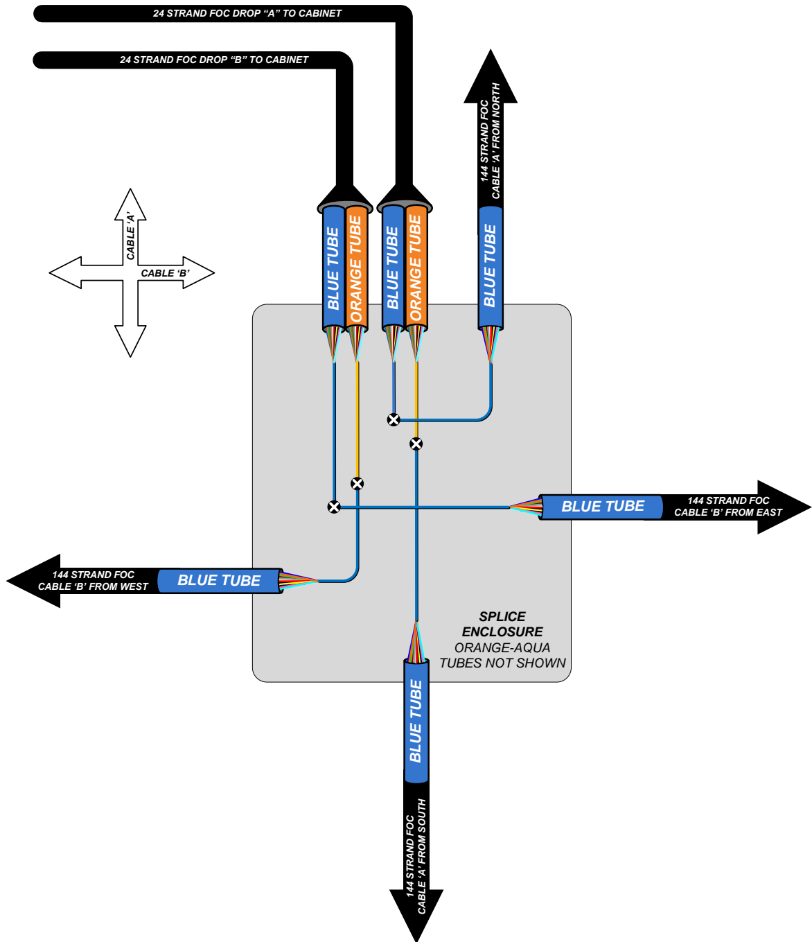
Figure 12.10 Splicing Orientation – 4 Cables
