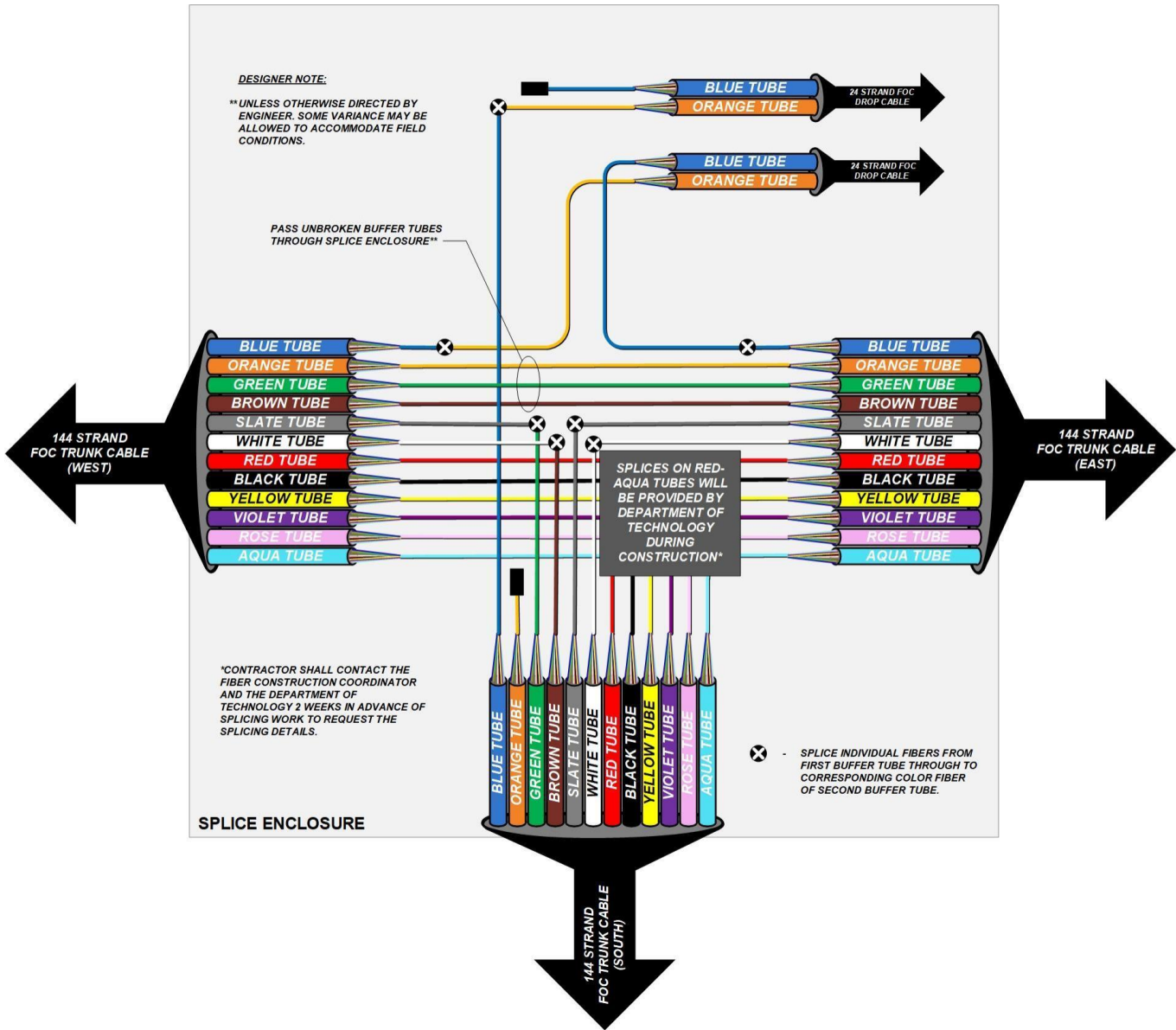
Figure 12.5 Typical Splicing Diagram – 3 cables
