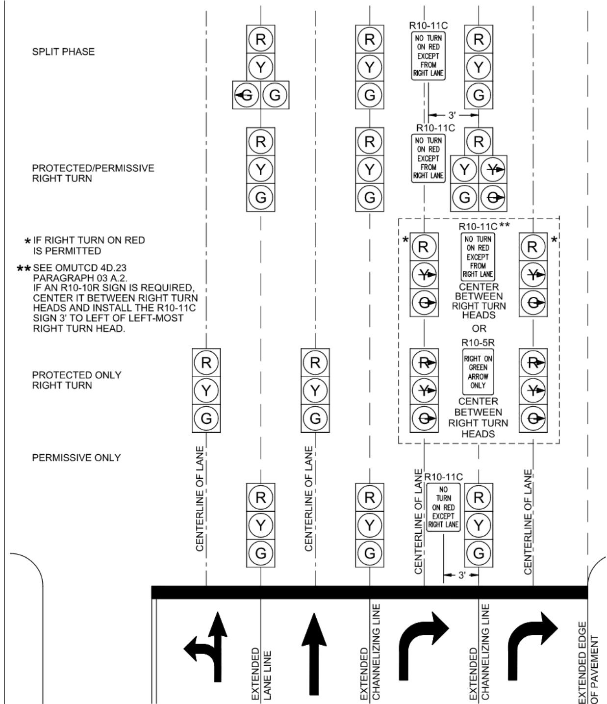
Figure 5.26 Vehicular Signal Head Alignment Four Approach Lanes Configuration F
