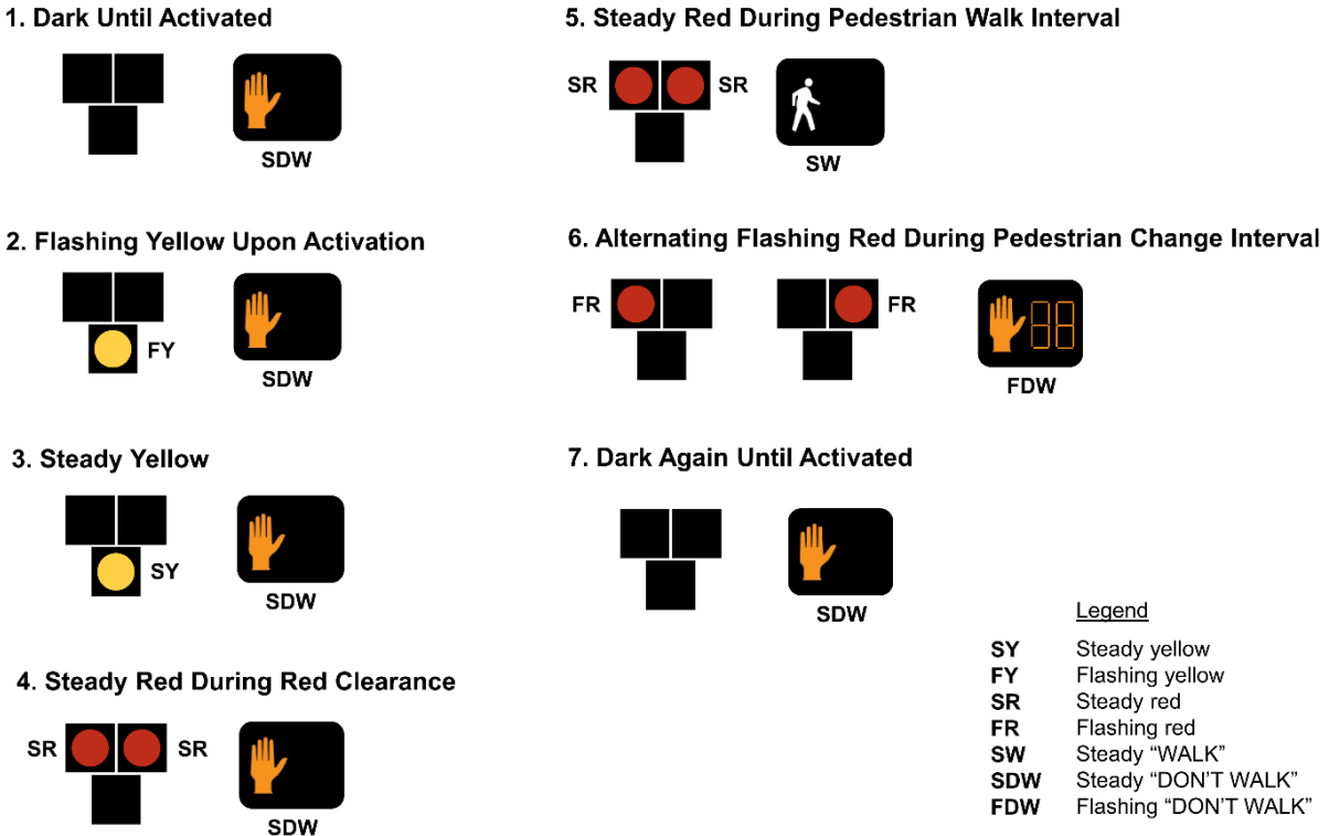
Figure 16.4 Sequence for a Pedestrian Hybrid Beacon
