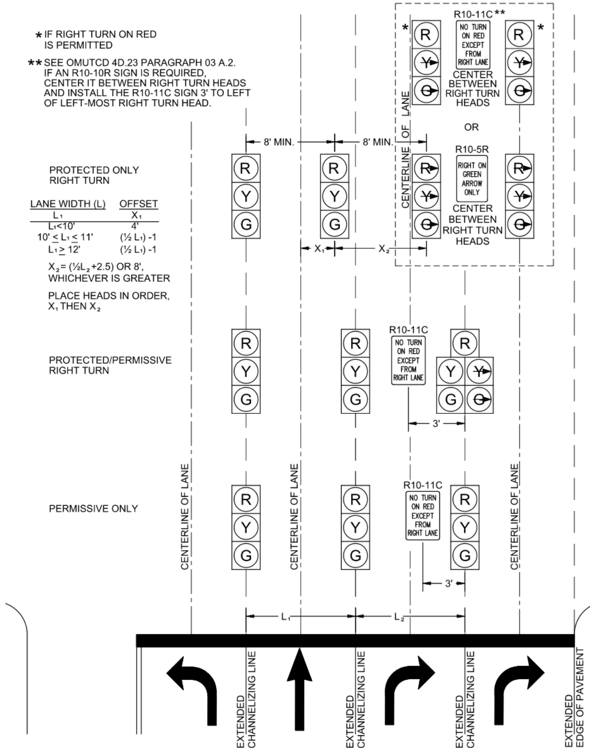
Figure 5.25 Vehicular Signal Head Alignment Four Approach Lanes Configuration E (2 of 2)
