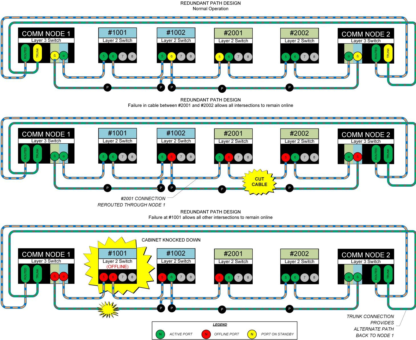
Figure 12.3 Fiber Optic Redundancy Scenarios
