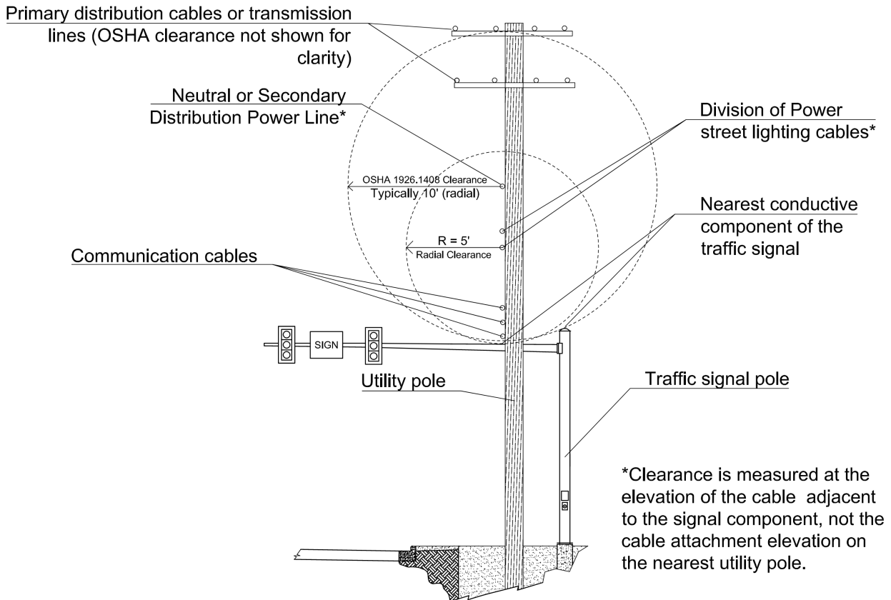
Figure 4.3 Overhead Utility Clearance Illustration (Mast Arm Cross-section View)
