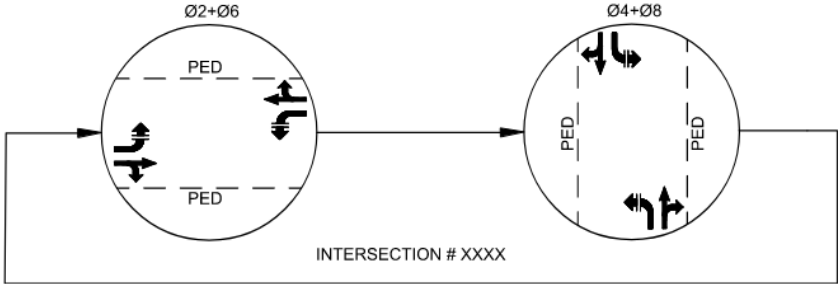
Figure 15.6 2 Phase Example East-West Mainline
