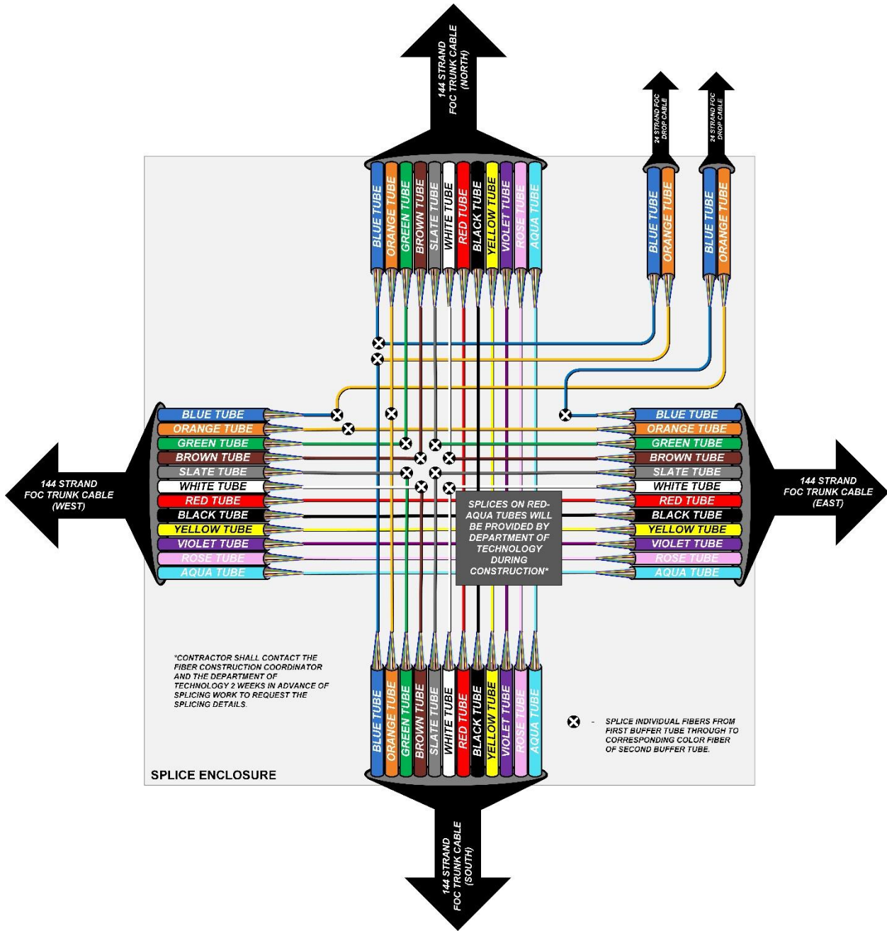
Figure 12.6 Typical Splicing Diagram – 4 cables
