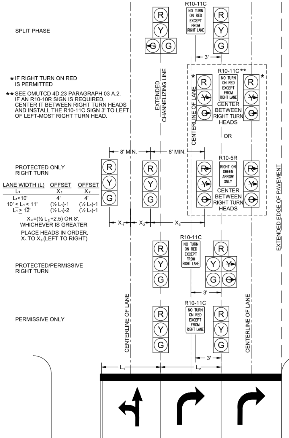
Figure 5.17 Vehicular Signal Head Alignment Three Approach Lanes Configuration G
