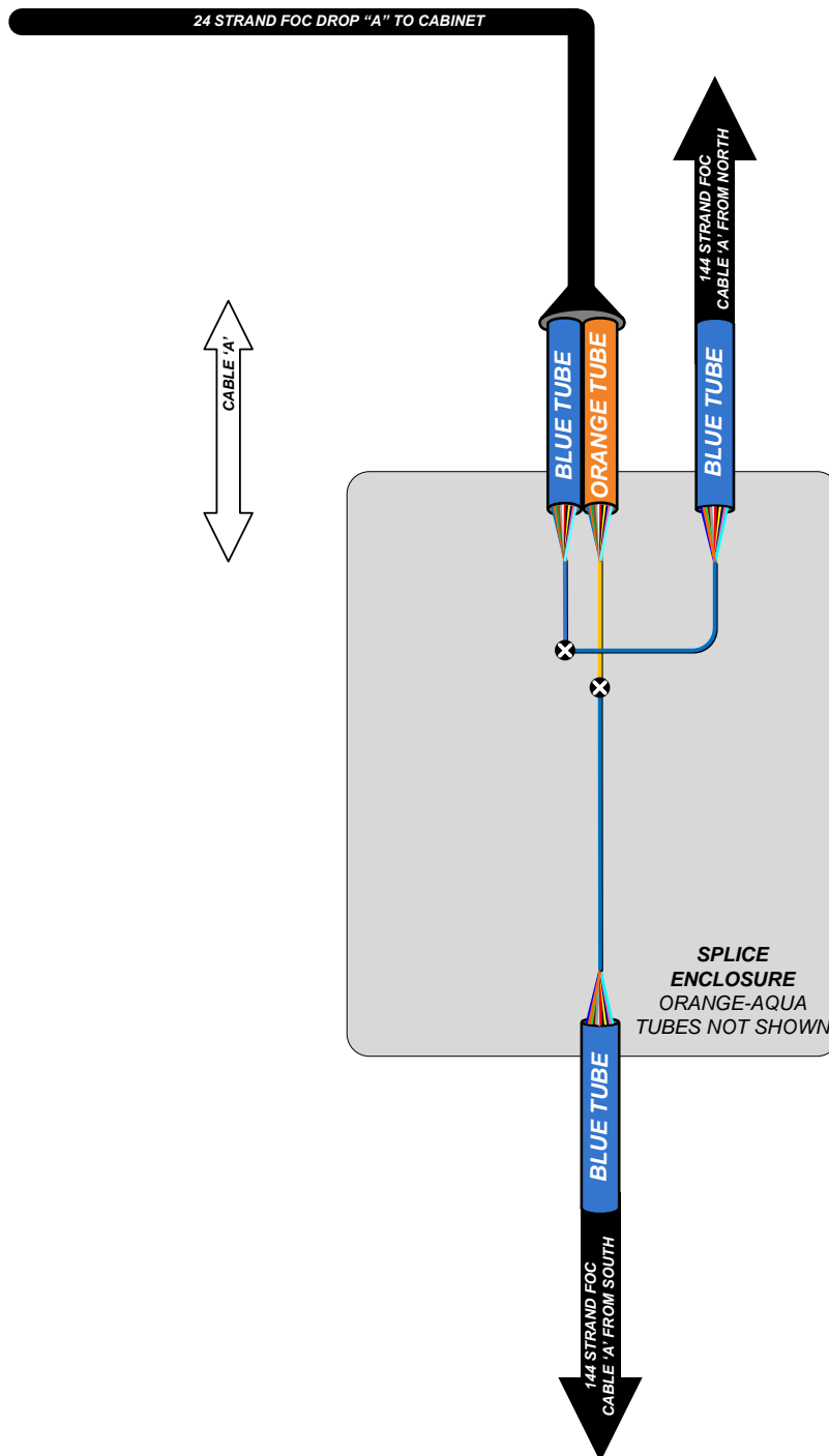
Figure 12.8 Splicing Orientation – 2 cables – North/South
