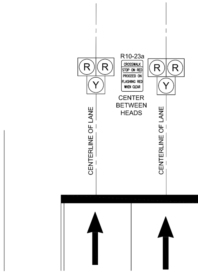
Figure 16.5 Pedestrian Hybrid Beacon Head Alignment Mid-Block Crossing Two Approach Lanes
