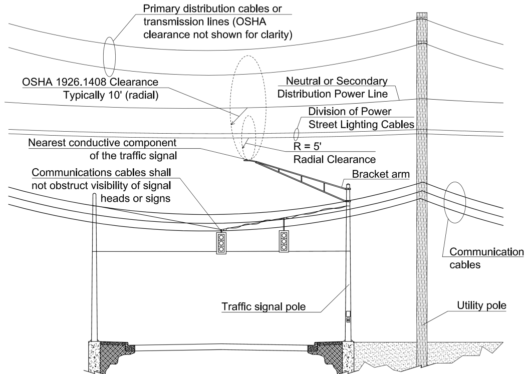
Figure 4.2 Overhead Utility Clearance Illustration (Strain Pole Cross-section View)
