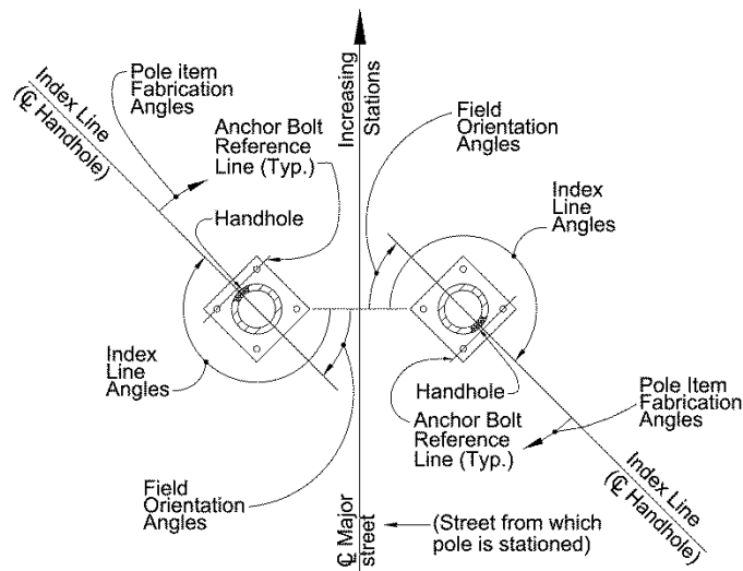
Figure 4.7 Typical Strain Pole and Pedestal Fabrication and Orientation Data
