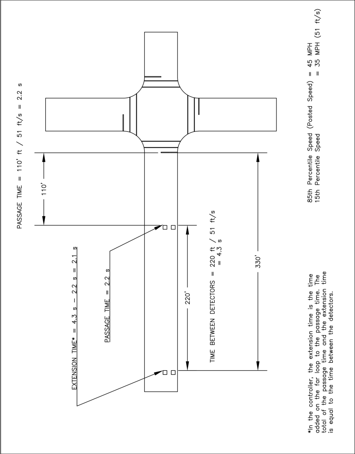
Figure 15.5 Dilemma Zone Example #1
