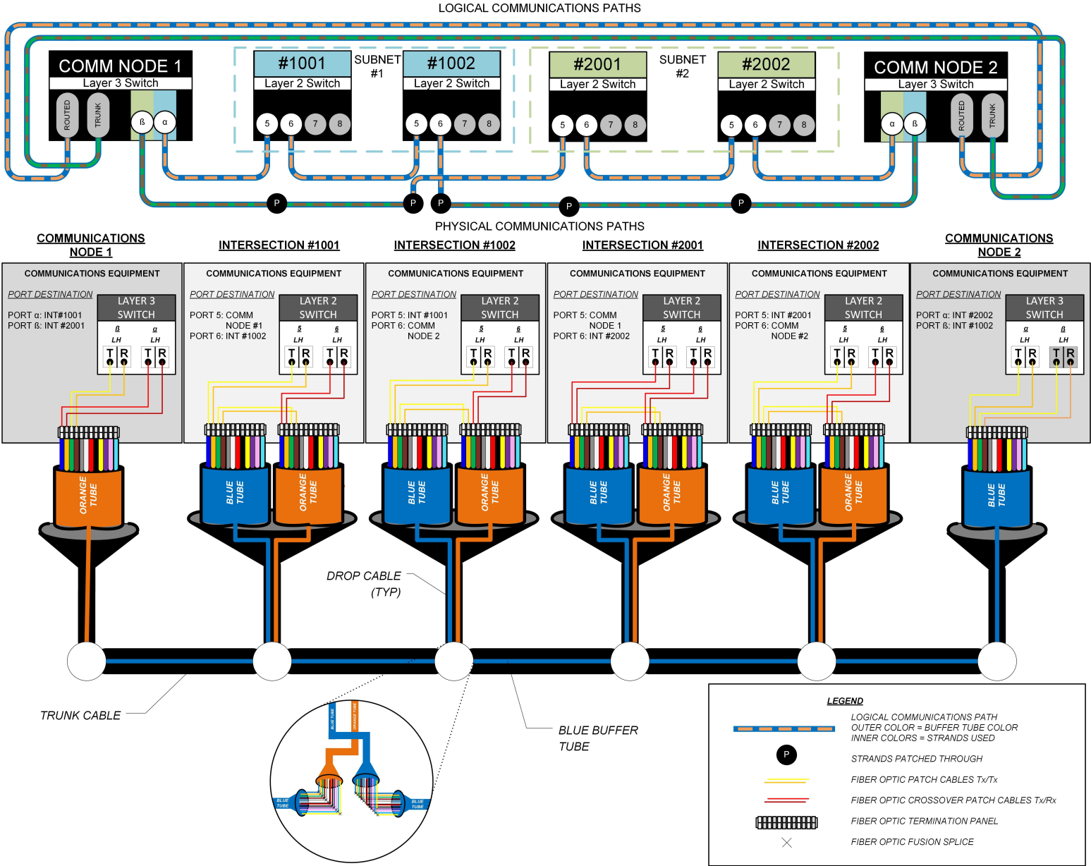
Figure 12.2 Fiber Optic Redundancy Communications Paths
