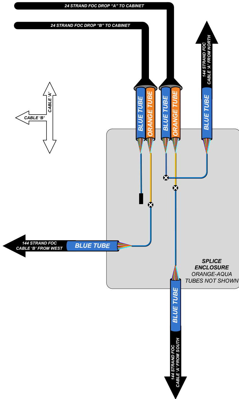
Figure 12.9 Splicing Orientation – 3 Cables
