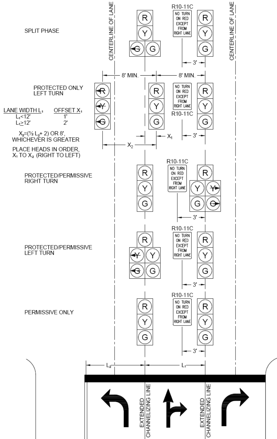
Figure 5.16 Vehicular Signal Head Alignment Three Approach Lanes Configuration F
