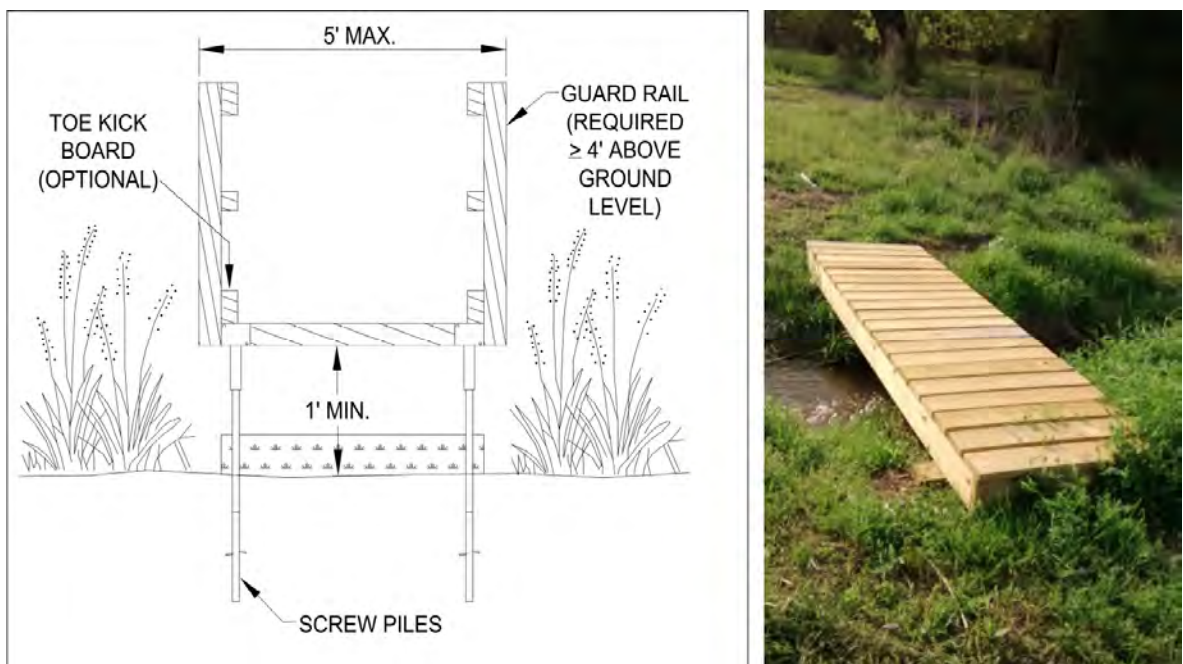
Figure 13. Boardwalk Cross Section Design Plan (L) and Stream Crossing Example (R)
